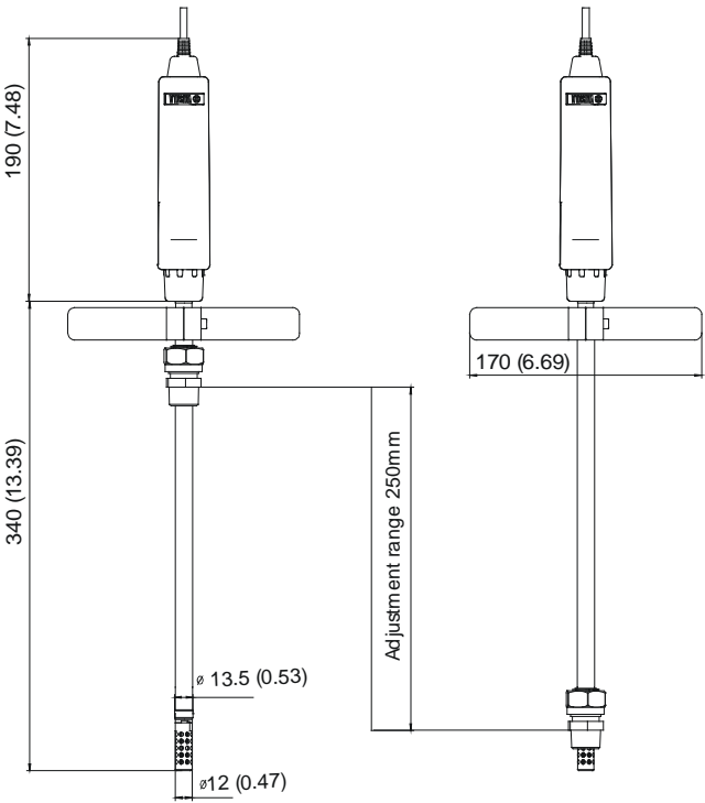
Figure 22 MMP78 Probe
