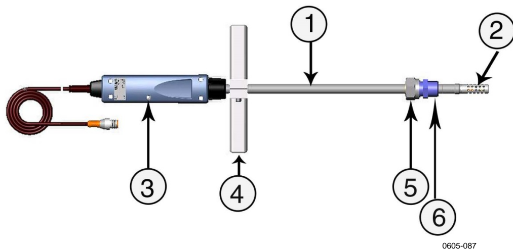
Figure 2 MMP78 Probe
