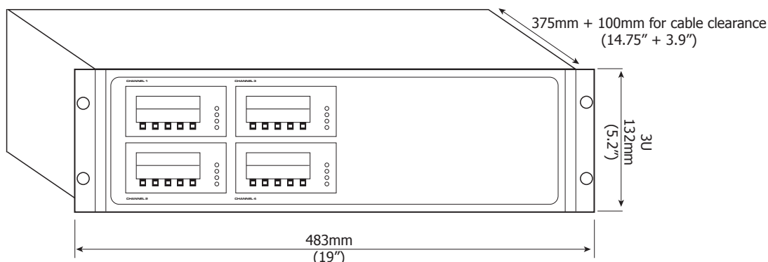
Figure 5 Dimensions of the Control Unit
