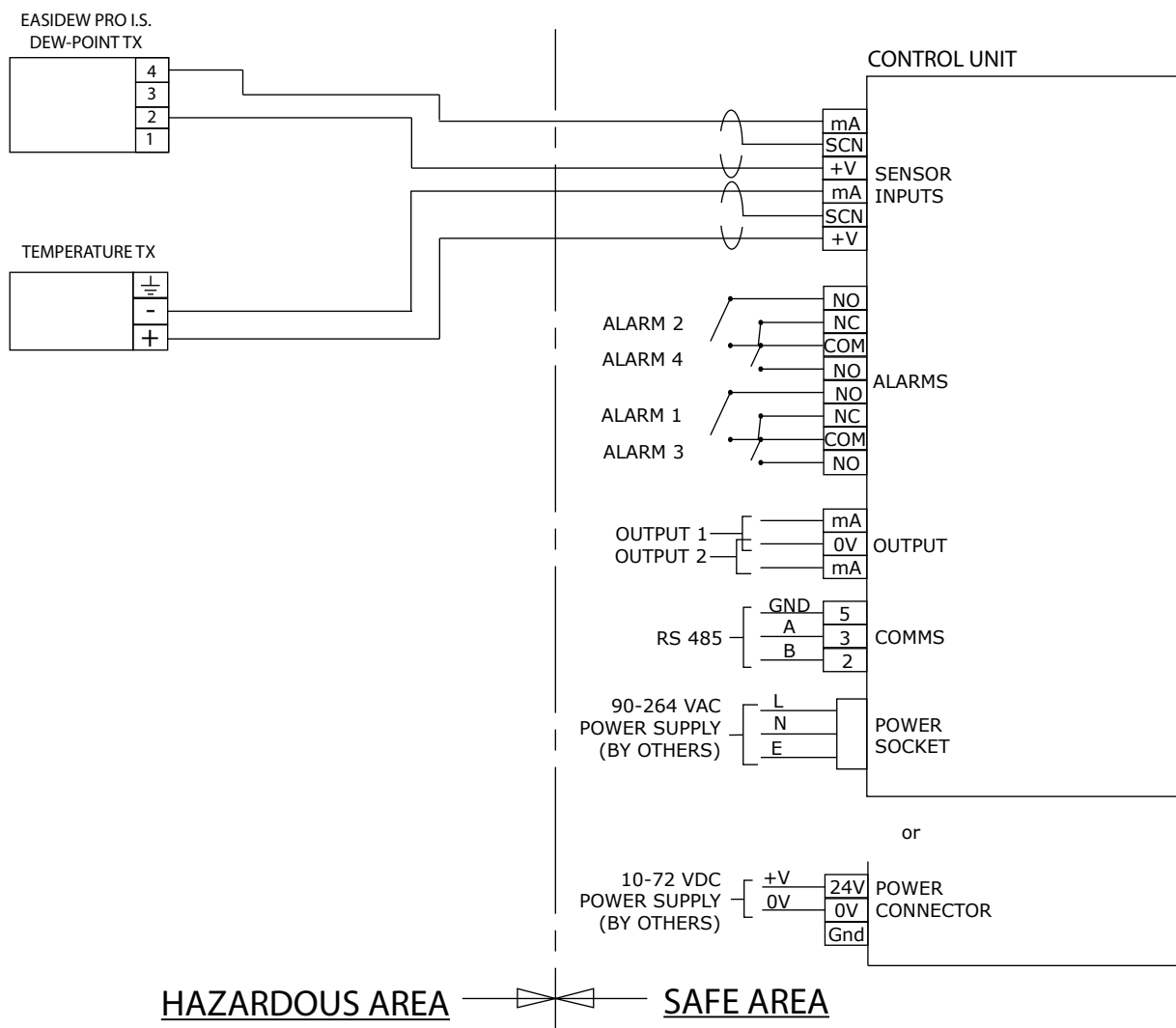
Figure 8 Overall Wiring Arrangement
