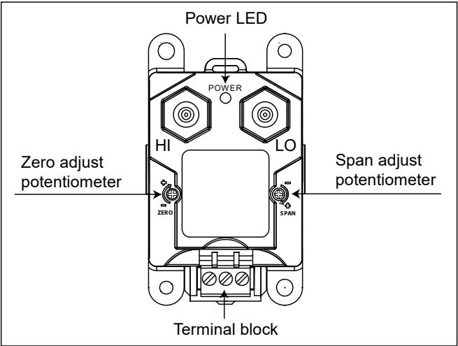
Figure 2 PDT101 Transmitter
