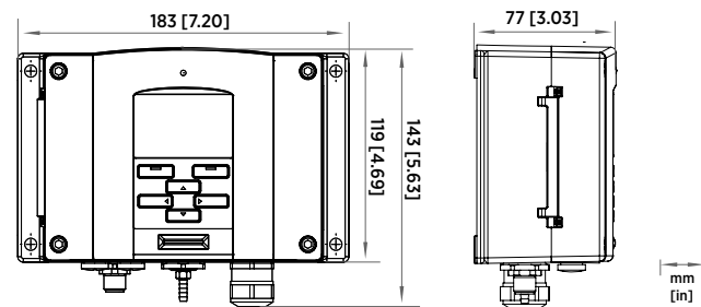
PTB330 dimensions
