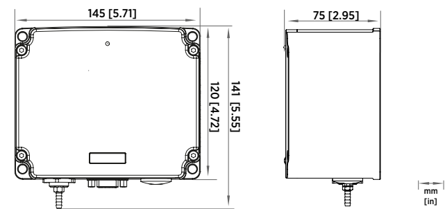
PTB330AWS dimensions
