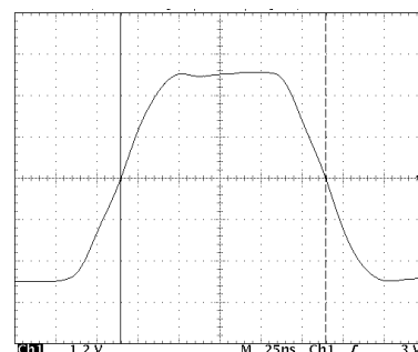
125ns Minimum Pulse Width, 6000V Output (25ns/Div horizontal scale, 1.2kV/Div vertical scale)
