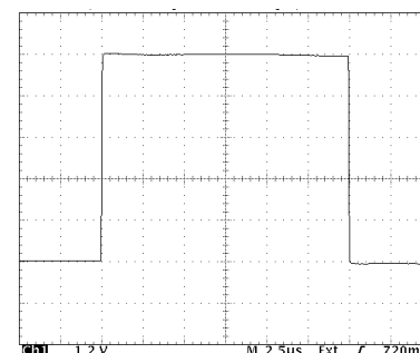
Typical Output Waveform, 6000V Output (2.5μs/Div horizontal scale, 1.2kV/Div vertical scale)
