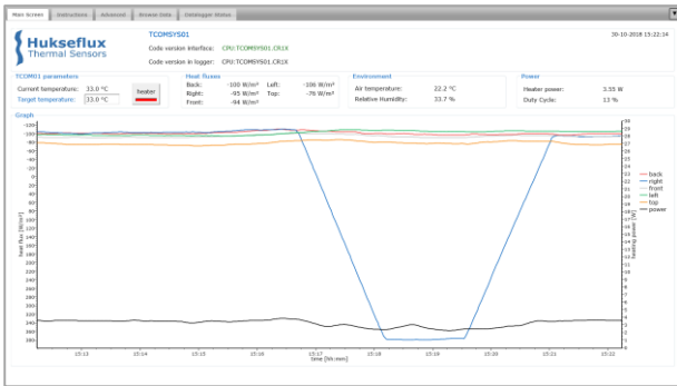
Figure 7 Example of TCOMSYS01 measurement. Five heat flux signals in [W/m 2 ] on the vertical axis, time [hr:min:s] on the horizontal axis. One side of TCOM01 is exposed to a strong radiative source. The system shows the radiative asymmetry
