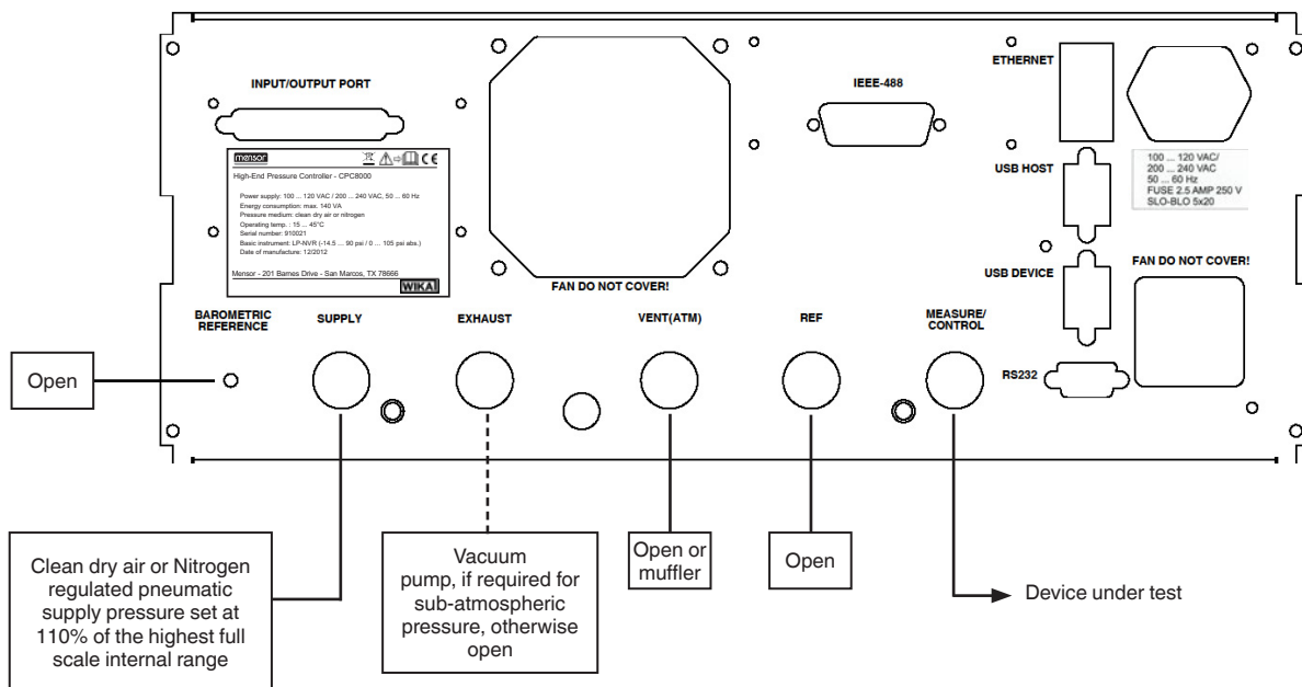
Figure 5.6 - Pneumatic Setup
