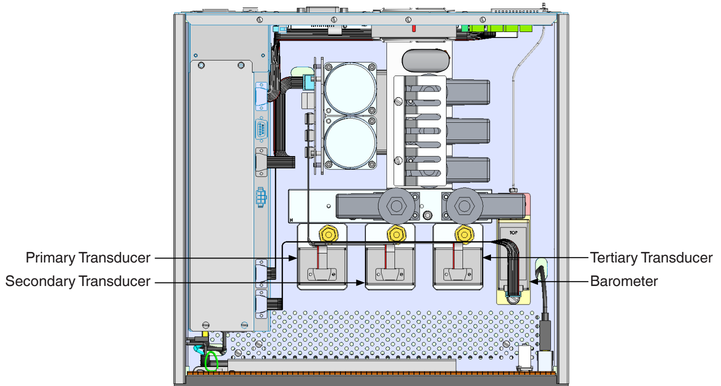
Figure 10.2.1 - Top View
